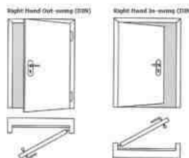
DIN Right means Hinge barrel is visible on right side that means a person will use Right hand to operate the door.
